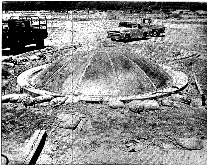
Fig. 10—Completed aluminum dome.
